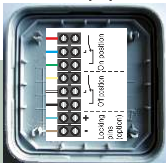
Interior view of the cover with wiring diagram
